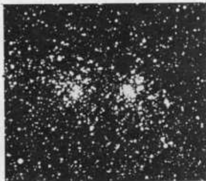
The brightest stars of the remote Double Cluster in Perseus are among the most luminous known, between ten thousand and a hundred thousand times as bright as the sun. Low power and wide field shows such clusters to best advantage.
